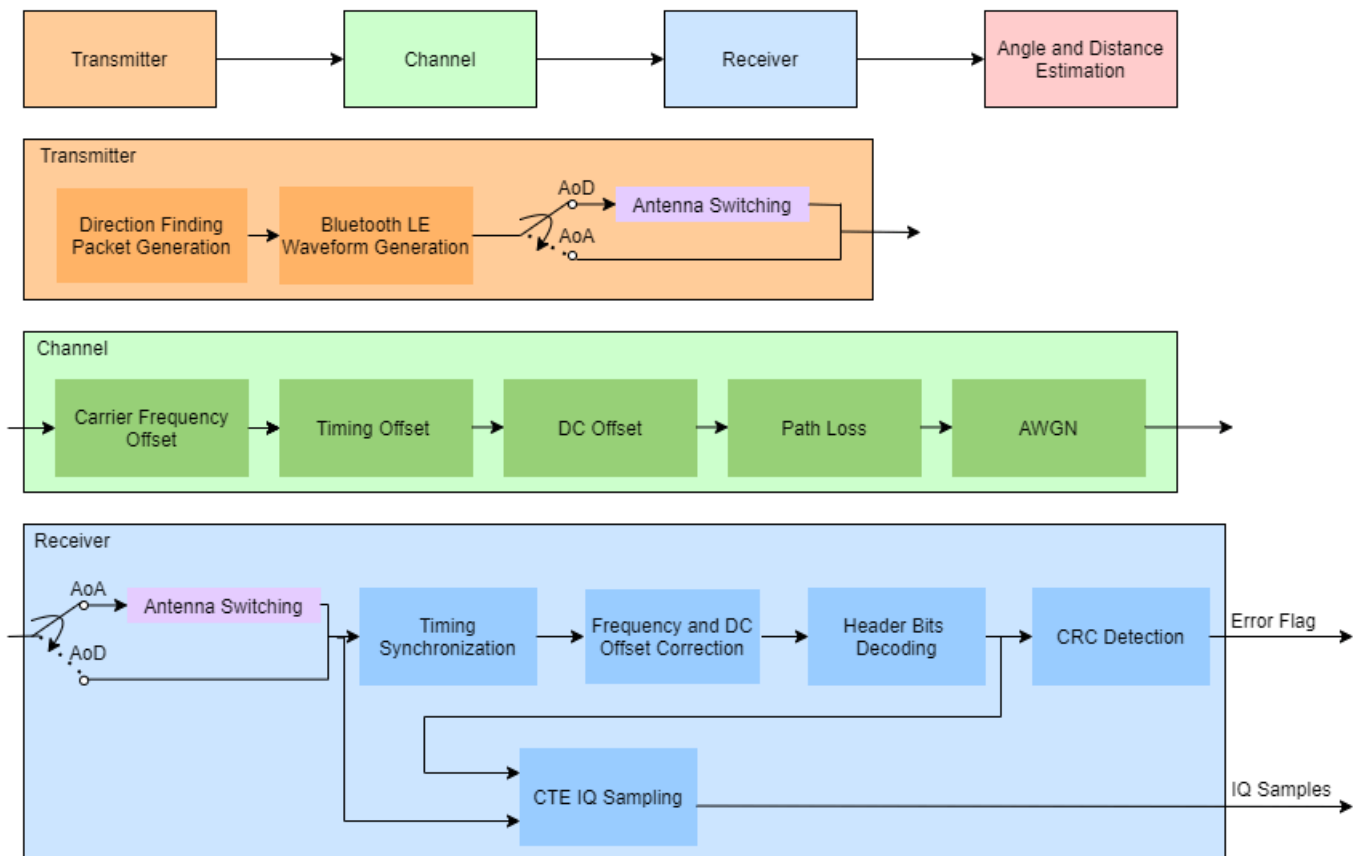
Bluetooth LE Node and Locator Chain
